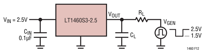
Figure 12. Response Time Test Circuit
